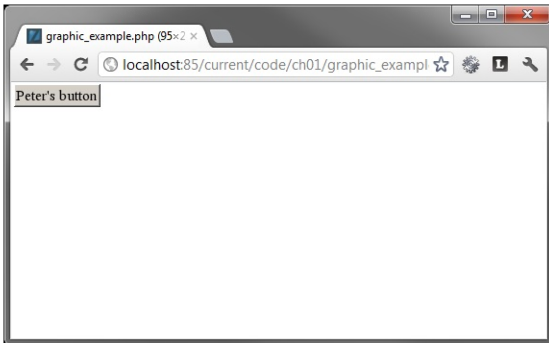
Figure 1-7. Button created
